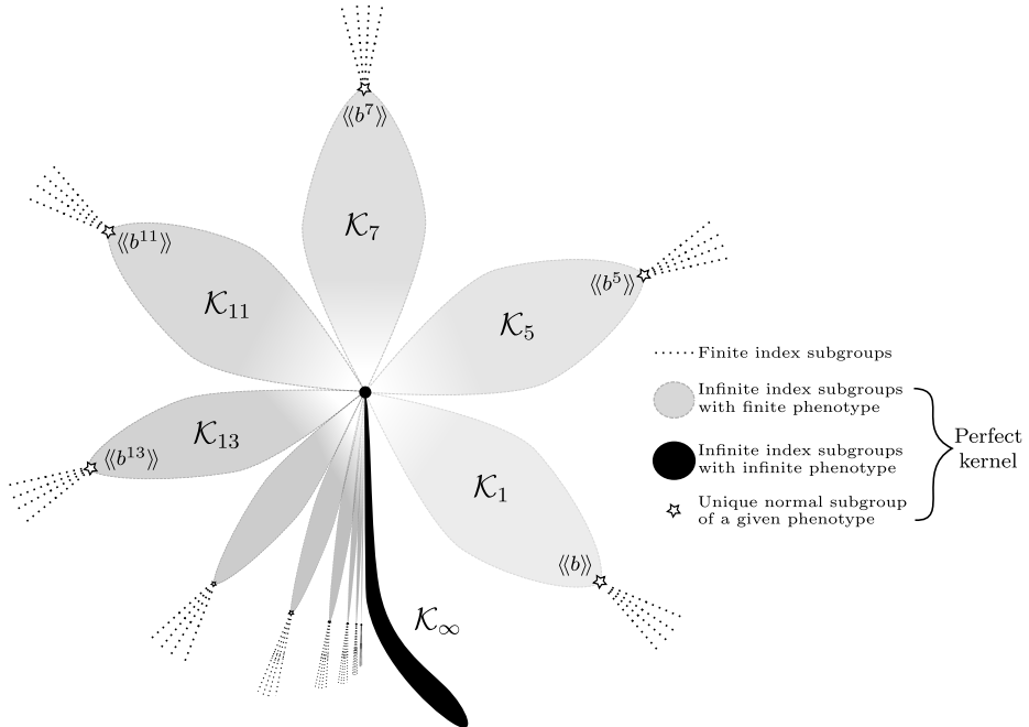
Figure 1. The space of subgroups of \text{BS}(2, 3)
