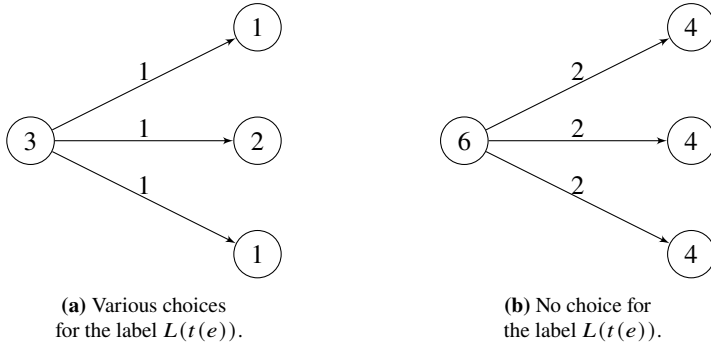
Figure 3. Two examples of (2, 3) -graphs.
